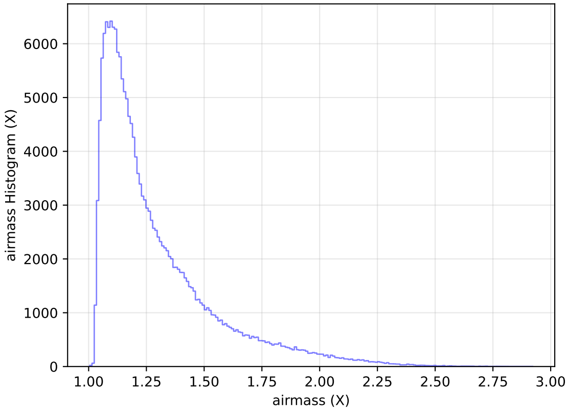
ddf_loaded_fl1_v3.4_10yrs WFD g band: airmass Histogram
