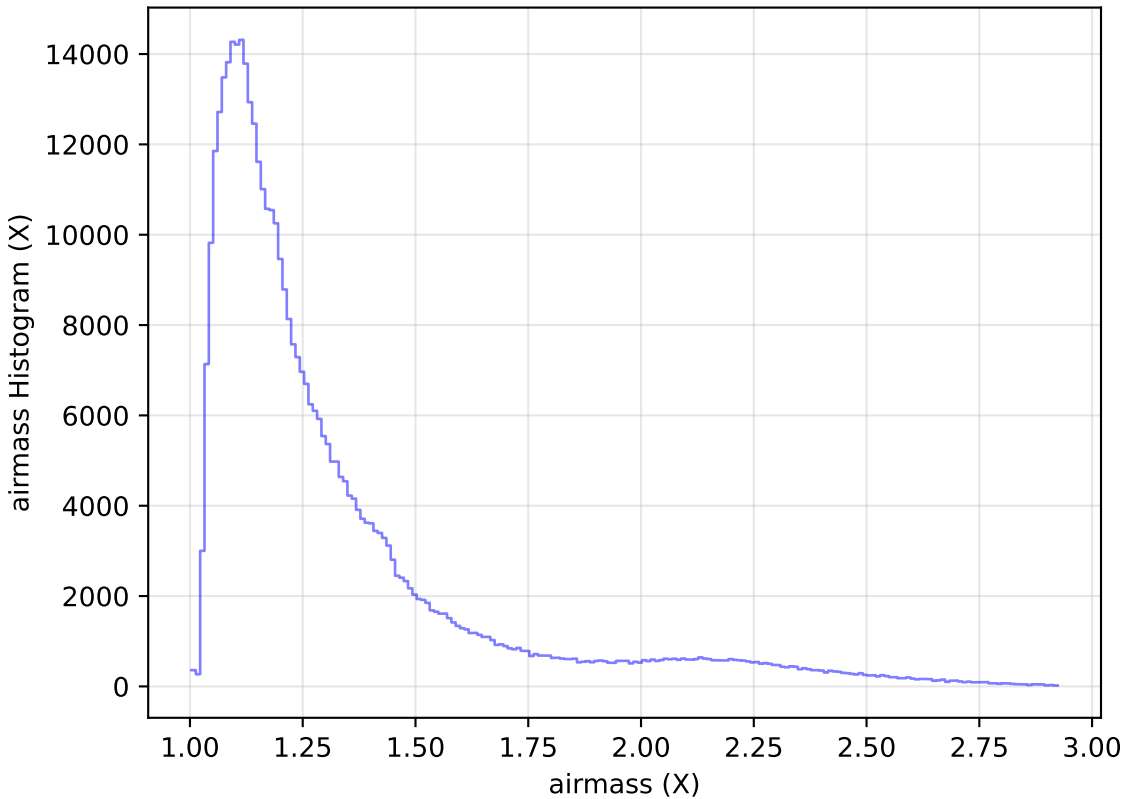
ddf_loaded_fl1_v3.4_10yrs All sky z band: airmass Histogram
