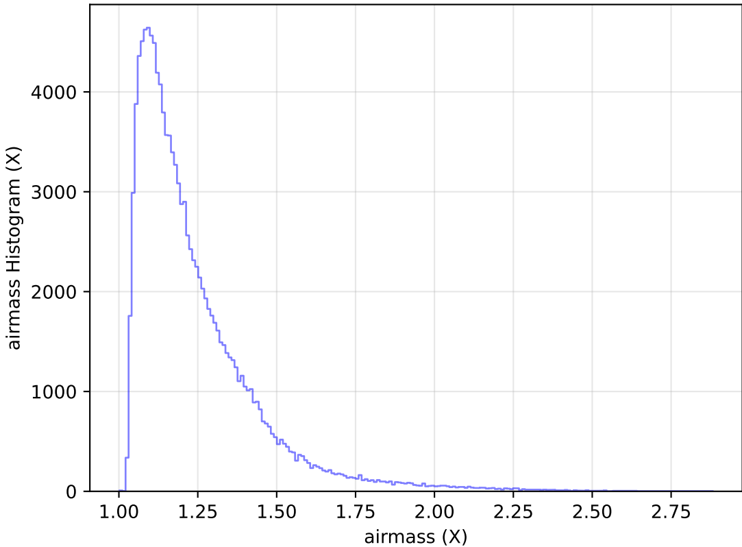
ddf_loaded_fl1_v3.4_10yrs All sky u band: airmass Histogram
