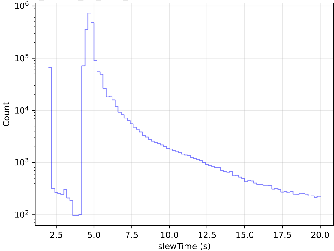
ddf_loaded_fl1_v3.4_10yrs All visits: Zoom Slew Time Histogram
