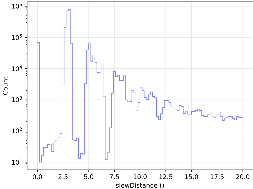
ddf_loaded_fl1_v3.4_10yrs All visits: Zoom Slew Distance Histogram
