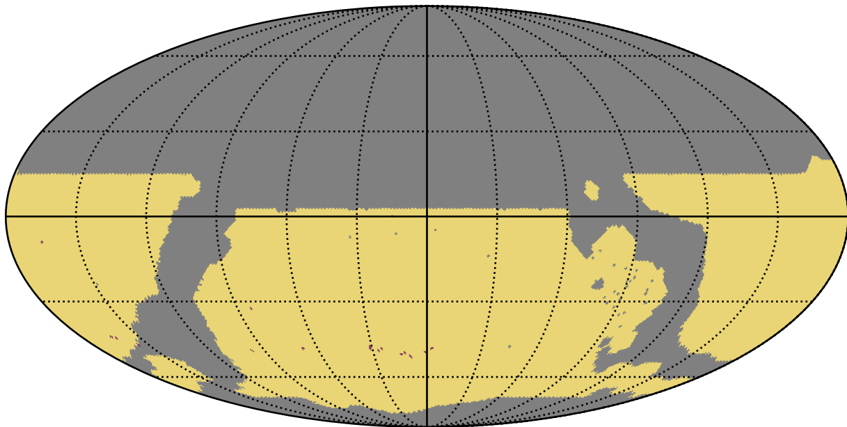
ddf_loaded_fl1_v3.4_10yrs WFD: RapidRevisits
