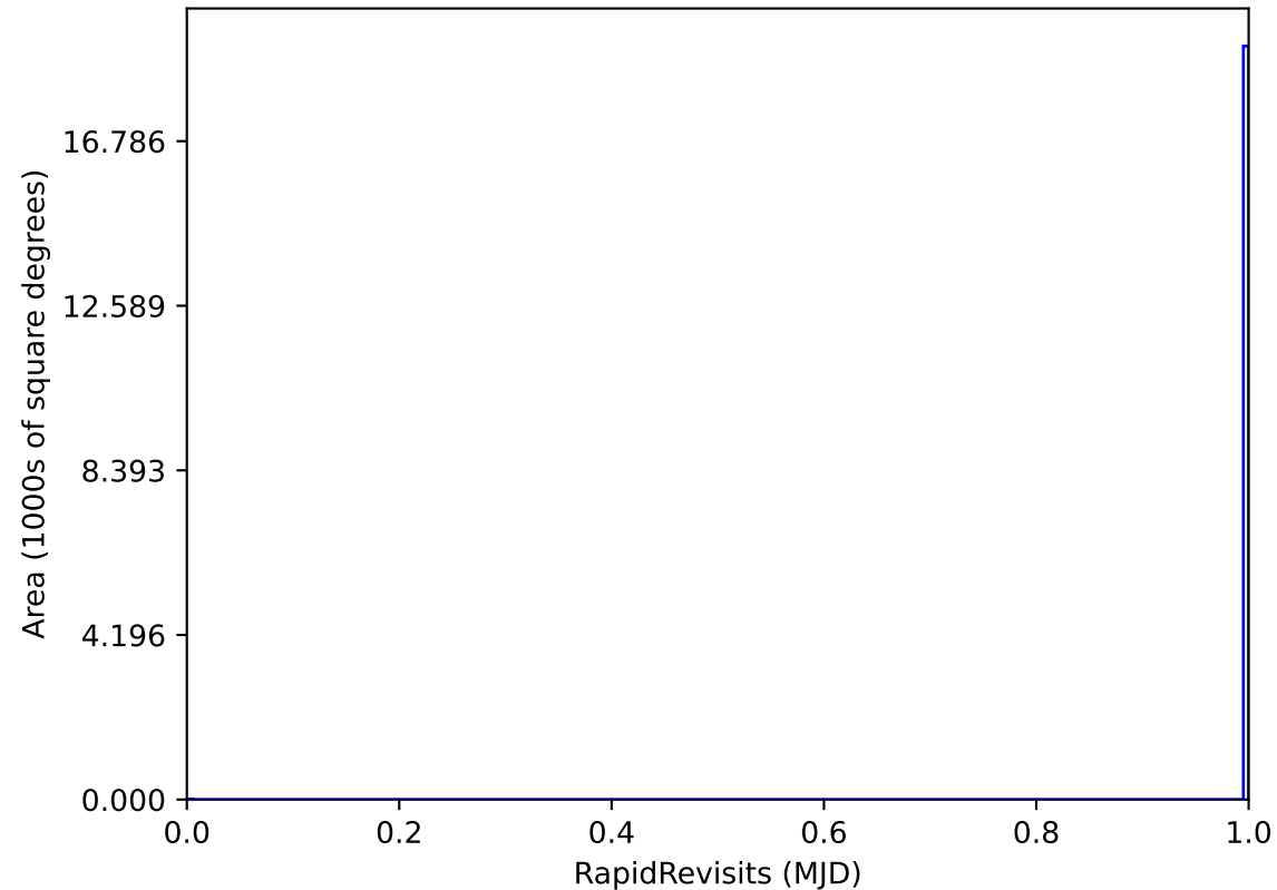
ddf_loaded_fl1_v3.4_10yrs WFD: RapidRevisits
