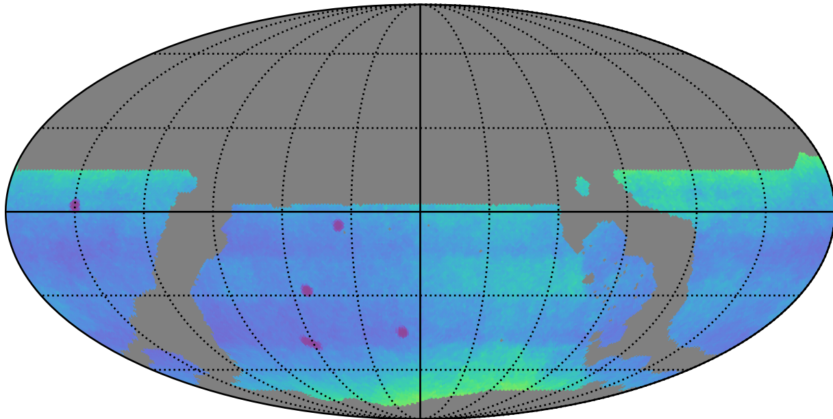
ddf_loaded_fl1_v3.4_10yrs WFD: Proper Motion Uncert @ 24.0
