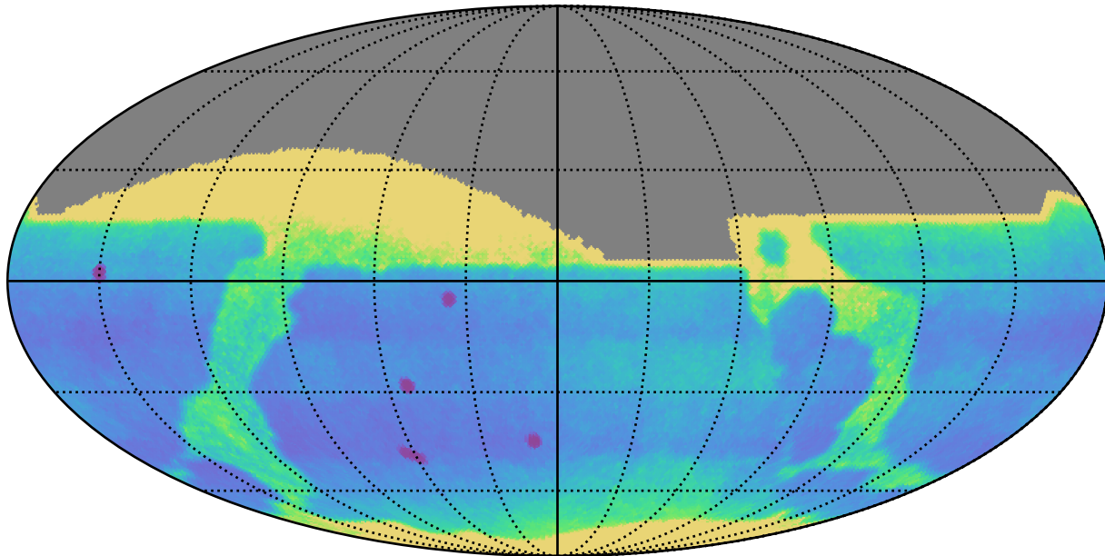
ddf_loaded_fl1_v3.4_10yrs All sky: Proper Motion Uncert @ 24.0
