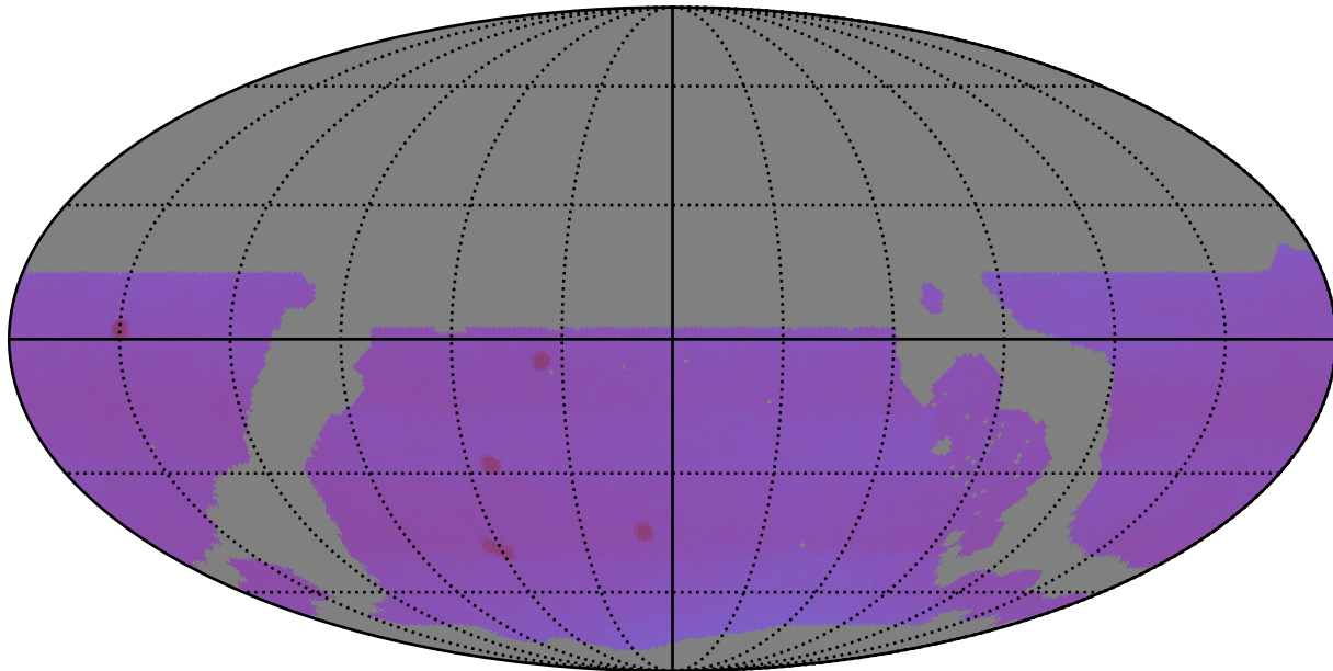
ddf_loaded_fl1_v3.4_10yrs WFD: Proper Motion Uncert @ 20.5
