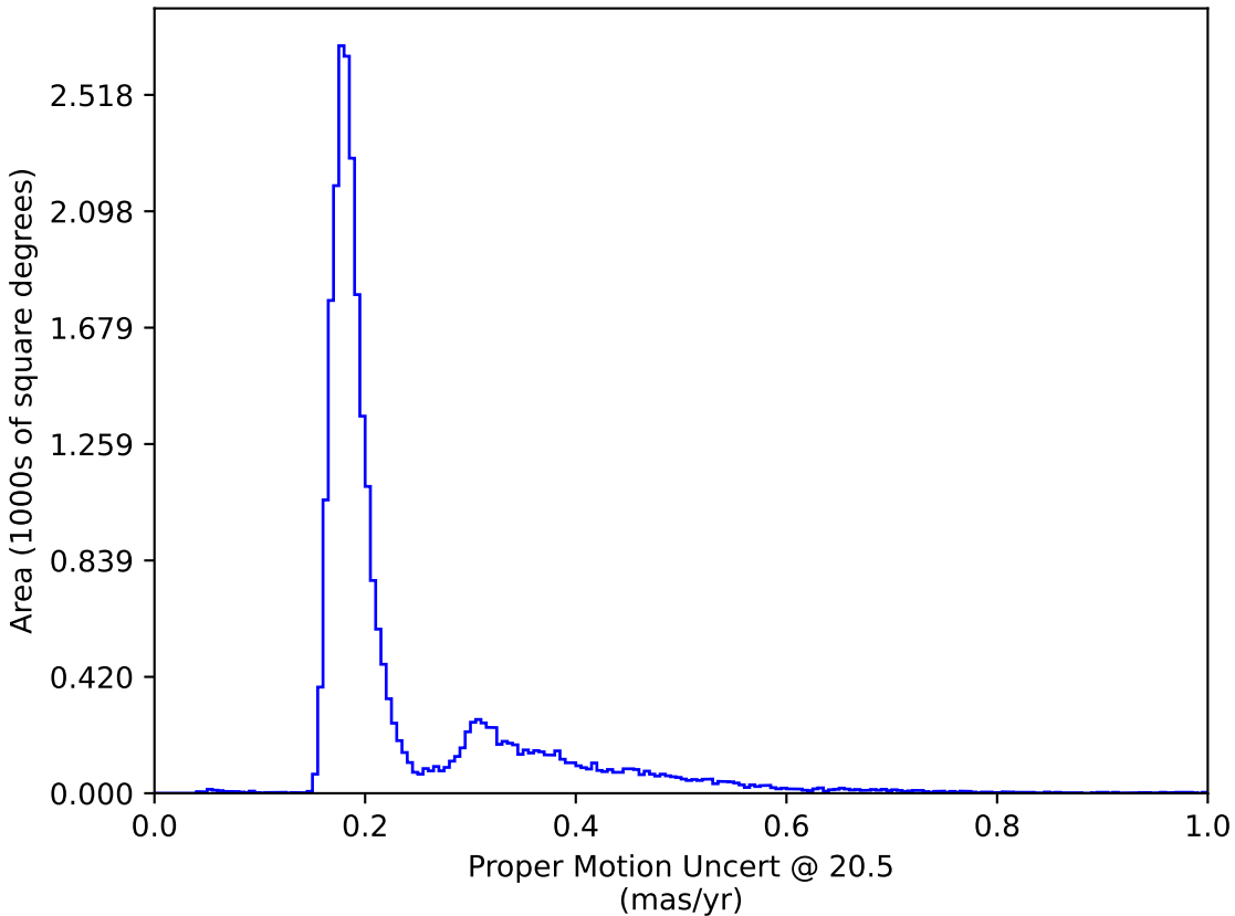
ddf_loaded_fl1_v3.4_10yrs All sky: Proper Motion Uncert @ 20.5
