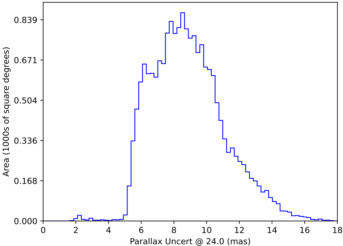
ddf_loaded_fl1_v3.4_10yrs WFD: Parallax Uncert @ 24.0
