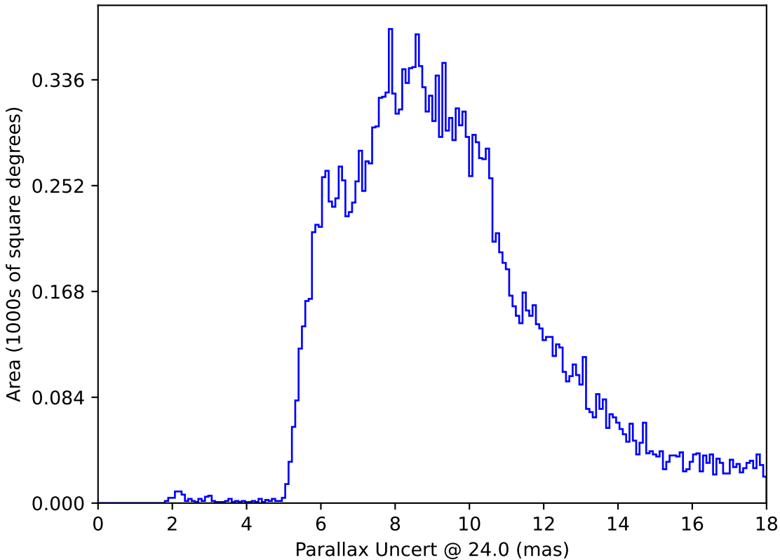
ddf_loaded_fl1_v3.4_10yrs All sky: Parallax Uncert @ 24.0
