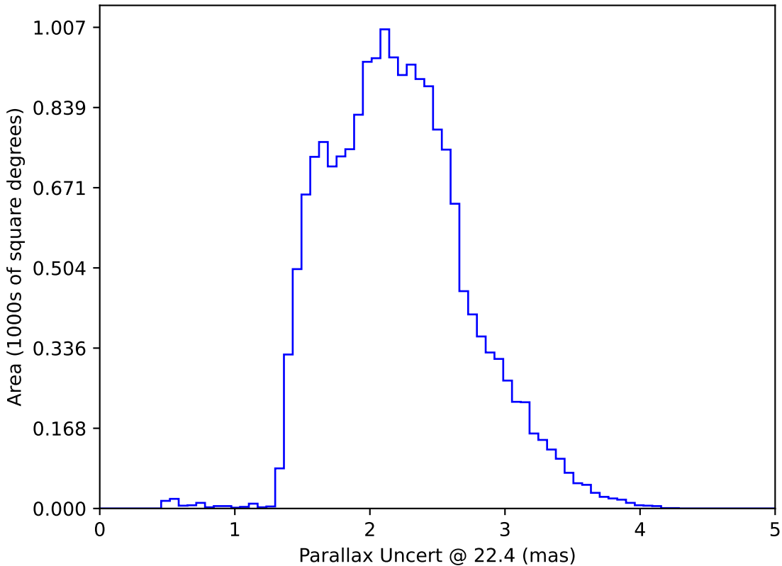
ddf_loaded_fl1_v3.4_10yrs WFD: Parallax Uncert @ 22.4
