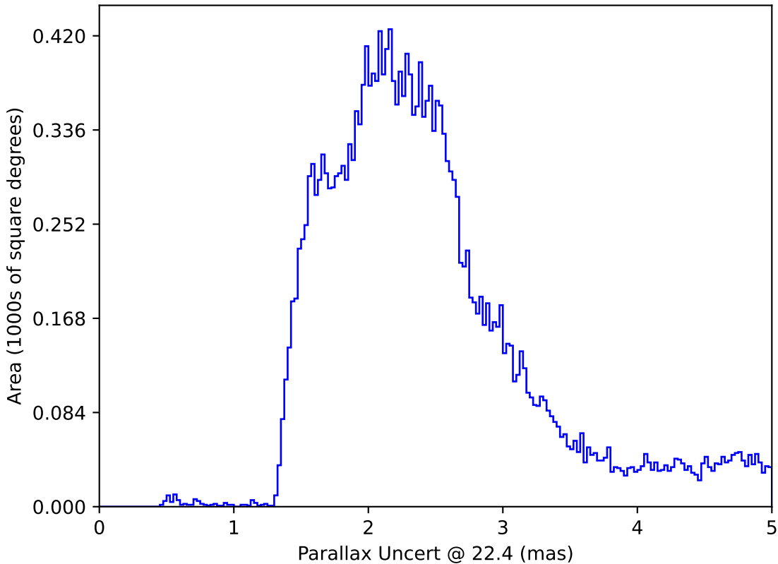
ddf_loaded_fl1_v3.4_10yrs All sky: Parallax Uncert @ 22.4
