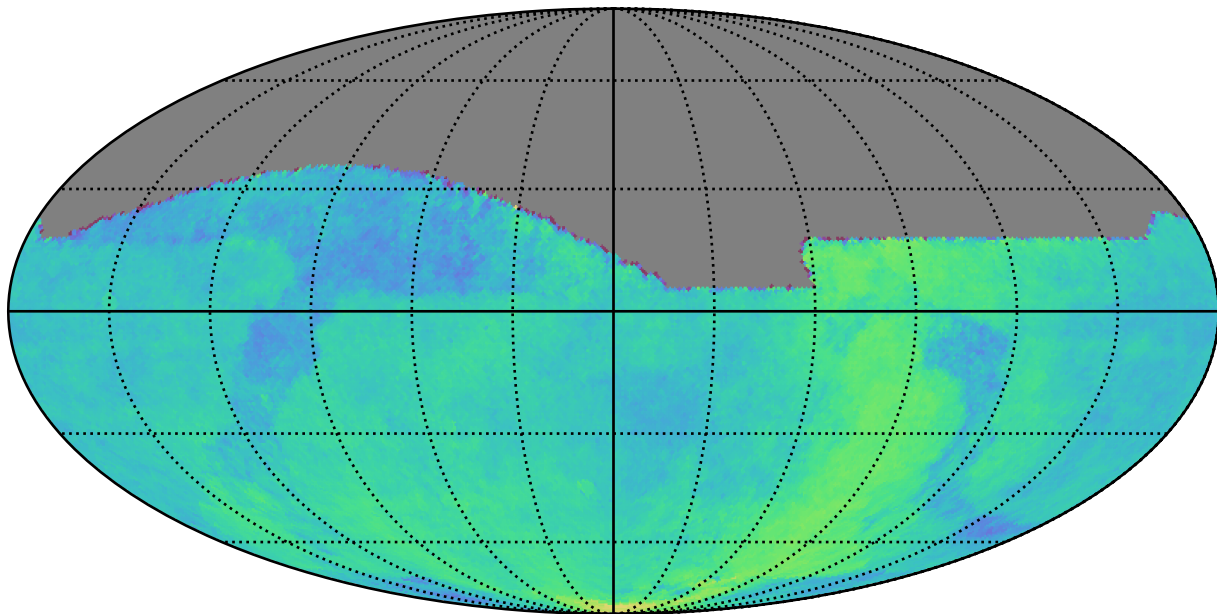
ddf_loaded_fl1_v3.4_10yrs All sky: Parallax Coverage @ 24.0
