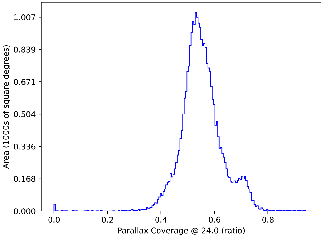
ddf_loaded_fl1_v3.4_10yrs All sky: Parallax Coverage @ 24.0
