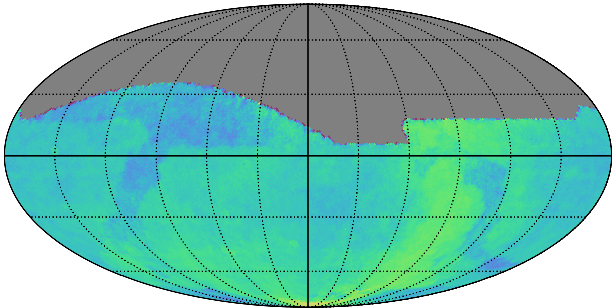
ddf_loaded_fl1_v3.4_10yrs All sky: Parallax Coverage @ 22.4
