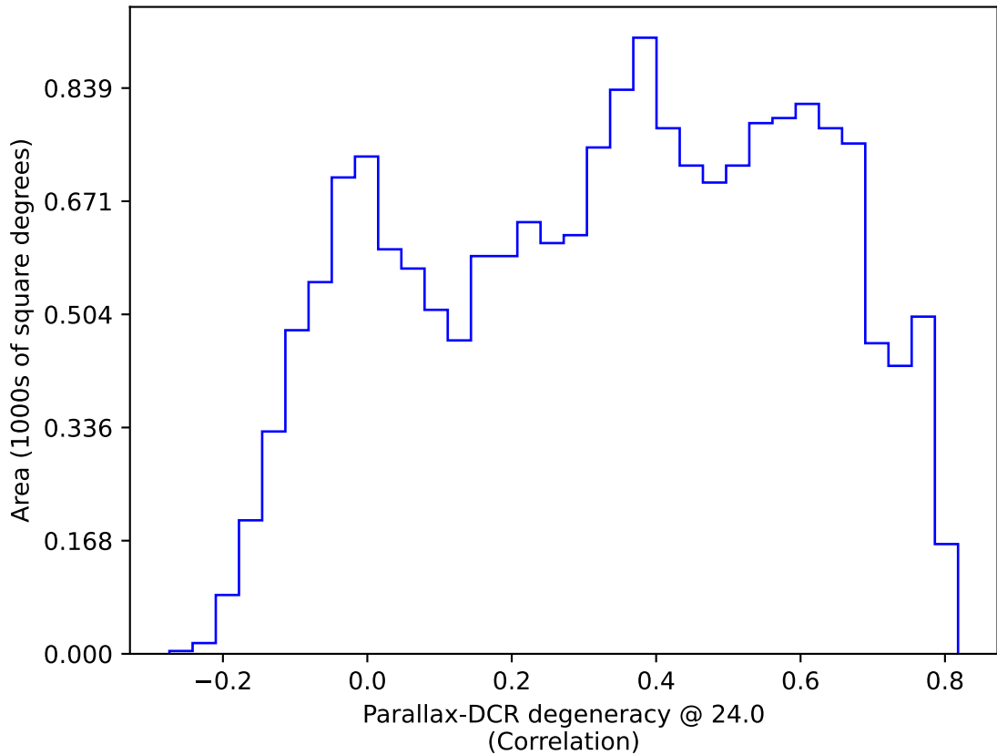
ddf_loaded_fl1_v3.4_10yrs WFD: Parallax-DCR degeneracy @ 24.0
