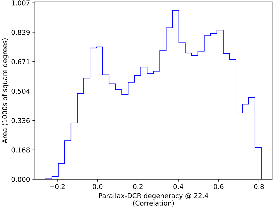
ddf_loaded_fl1_v3.4_10yrs WFD: Parallax-DCR degeneracy @ 22.4
