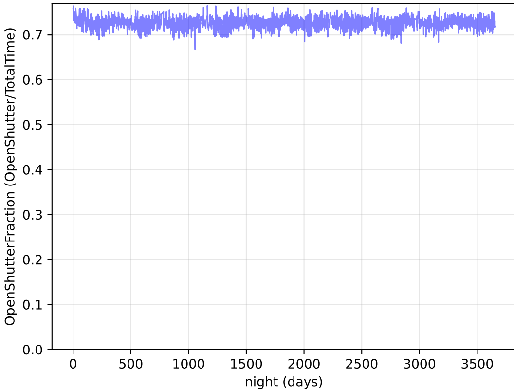
ddf_loaded_fl1_v3.4_10yrs Per night: OpenShutterFraction
