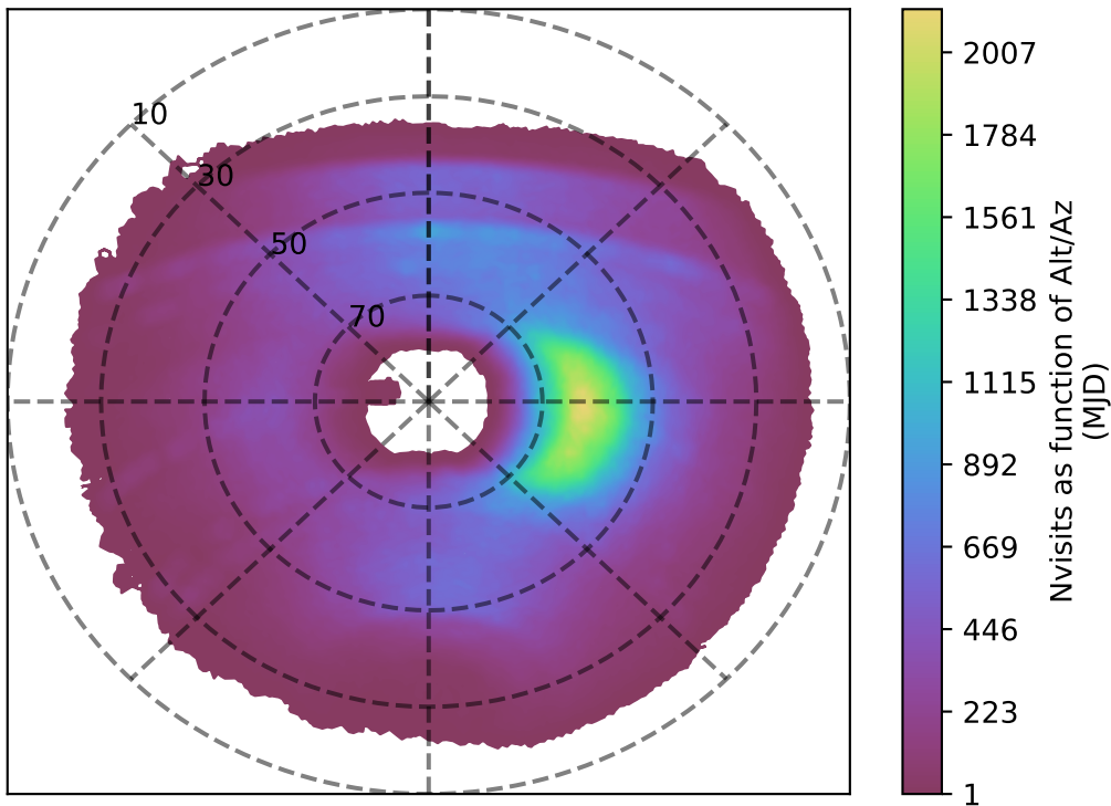
ddf_loaded_fl1_v3.4_10yrs y band: Nvisits as function of Alt/Az
