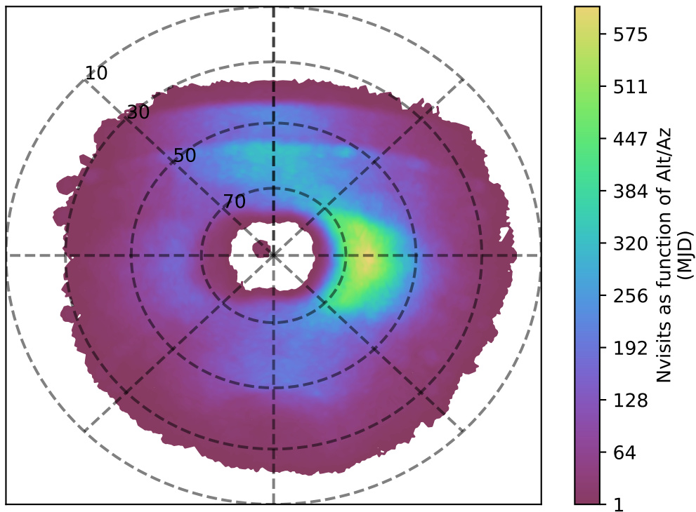
ddf_loaded_fl1_v3.4_10yrs u band: Nvisits as function of Alt/Az
