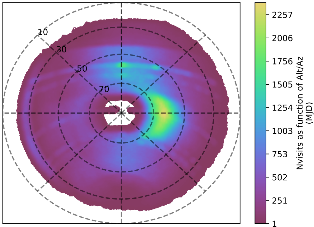
ddf_loaded_fl1_v3.4_10yrs r band: Nvisits as function of Alt/Az
