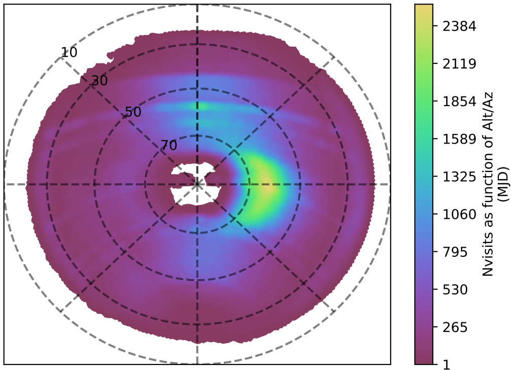
ddf_loaded_fl1_v3.4_10yrs i band: Nvisits as function of Alt/Az
