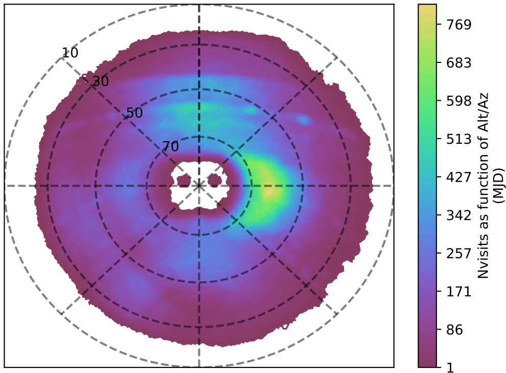
ddf_loaded_fl1_v3.4_10yrs g band: Nvisits as function of Alt/Az
