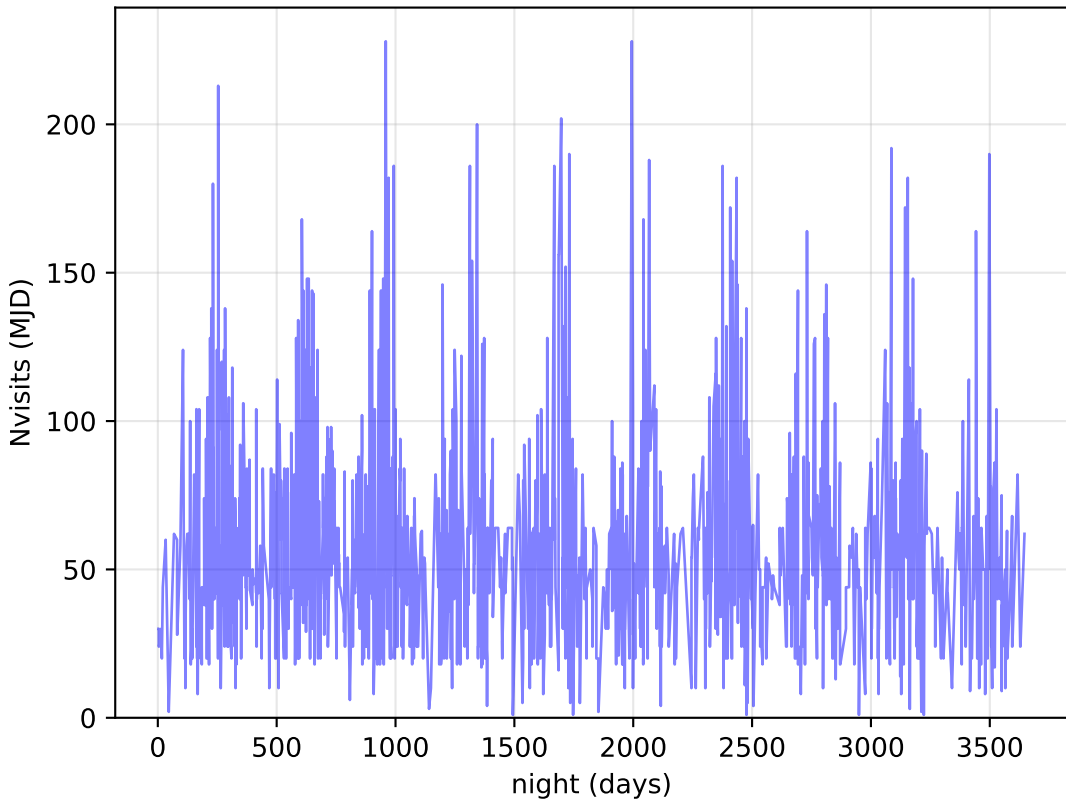
ddf_loaded_fl1_v3.4_10yrs DDF: Nvisits
