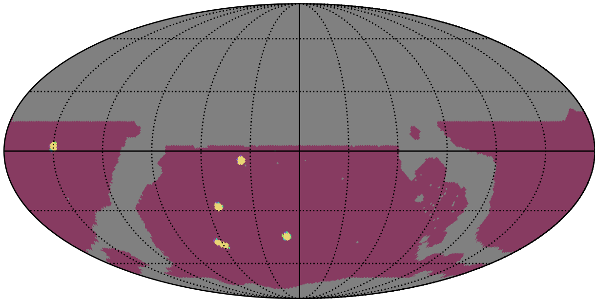
ddf_loaded_fl1_v3.4_10yrs WFD: NumberOfQuickRevisits
