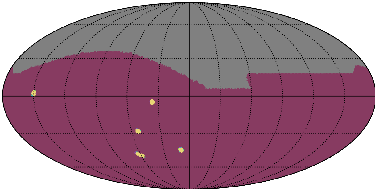
ddf_loaded_fl1_v3.4_10yrs All sky: NumberOfQuickRevisits
