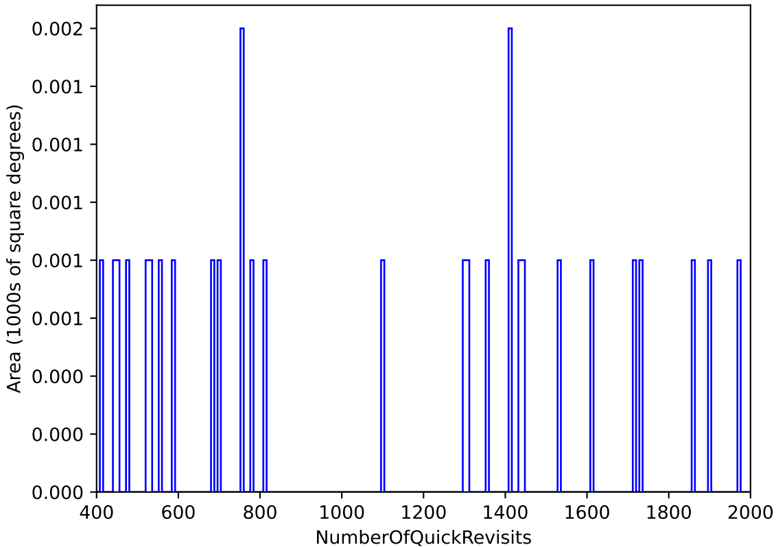
ddf_loaded_fl1_v3.4_10yrs All sky: NumberOfQuickRevisits
