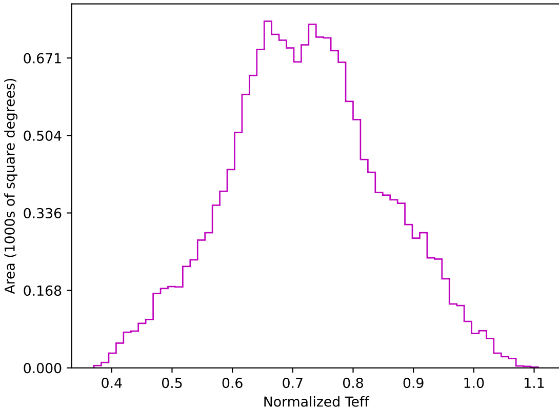
ddf_loaded_fl1_v3.4_10yrs WFD z band: Normalized Teff
