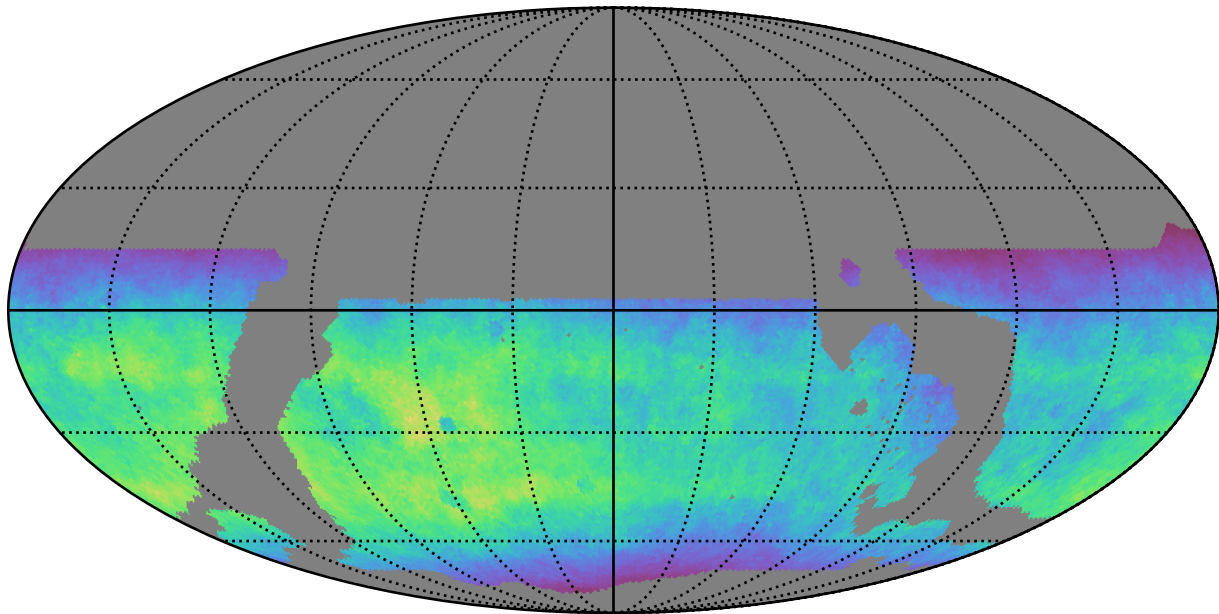
ddf_loaded_fl1_v3.4_10yrs WFD y band: Normalized Teff
