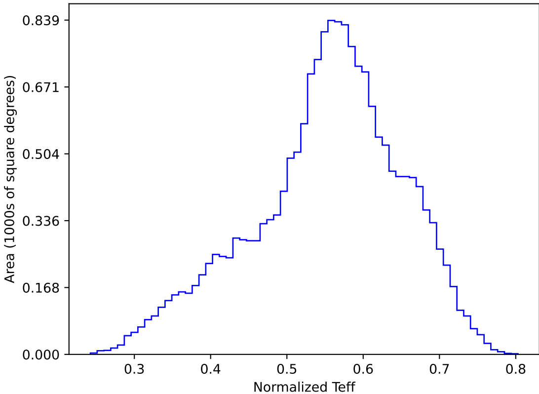
ddf_loaded_fl1_v3.4_10yrs WFD y band: Normalized Teff
