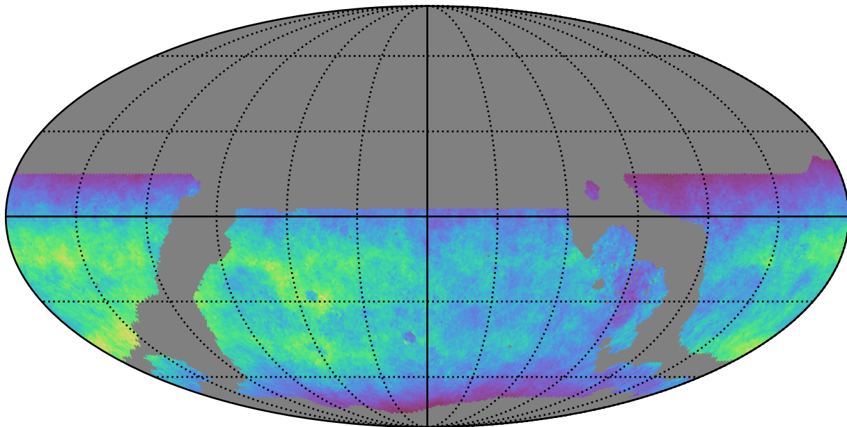
ddf_loaded_fl1_v3.4_10yrs WFD u band: Normalized Teff
