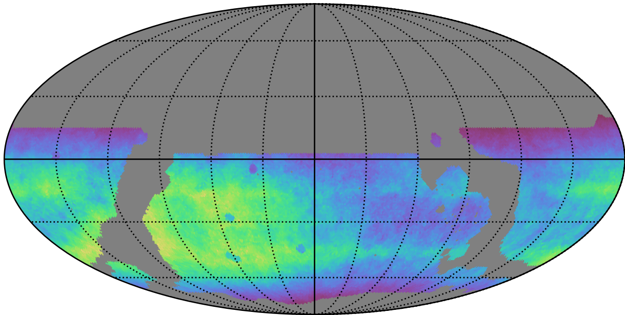
ddf_loaded_fl1_v3.4_10yrs WFD r band: Normalized Teff
