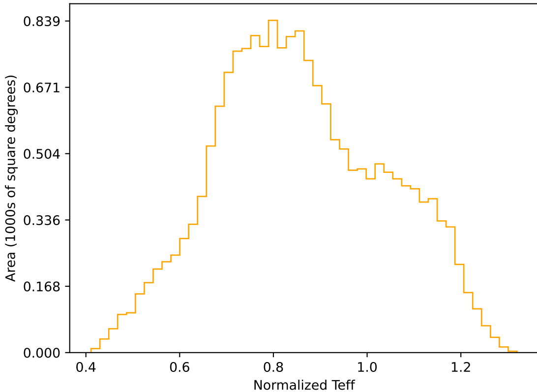
ddf_loaded_fl1_v3.4_10yrs WFD r band: Normalized Teff
