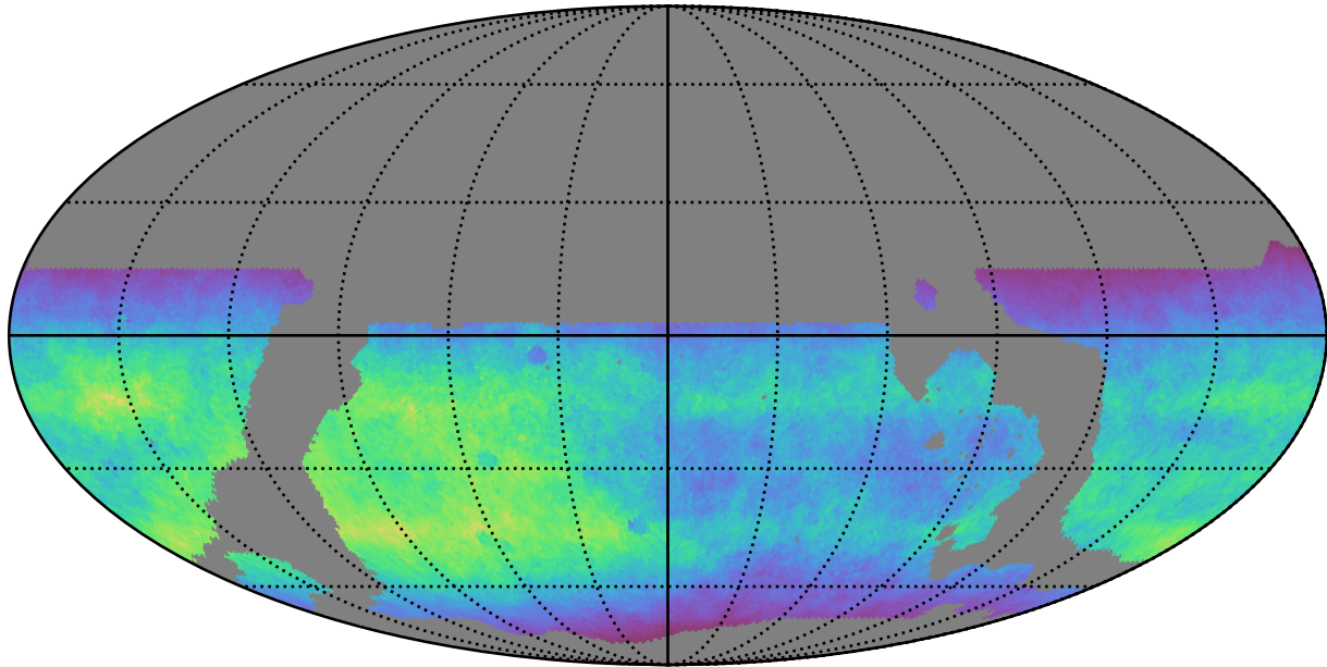
ddf_loaded_fl1_v3.4_10yrs WFD i band: Normalized Teff
