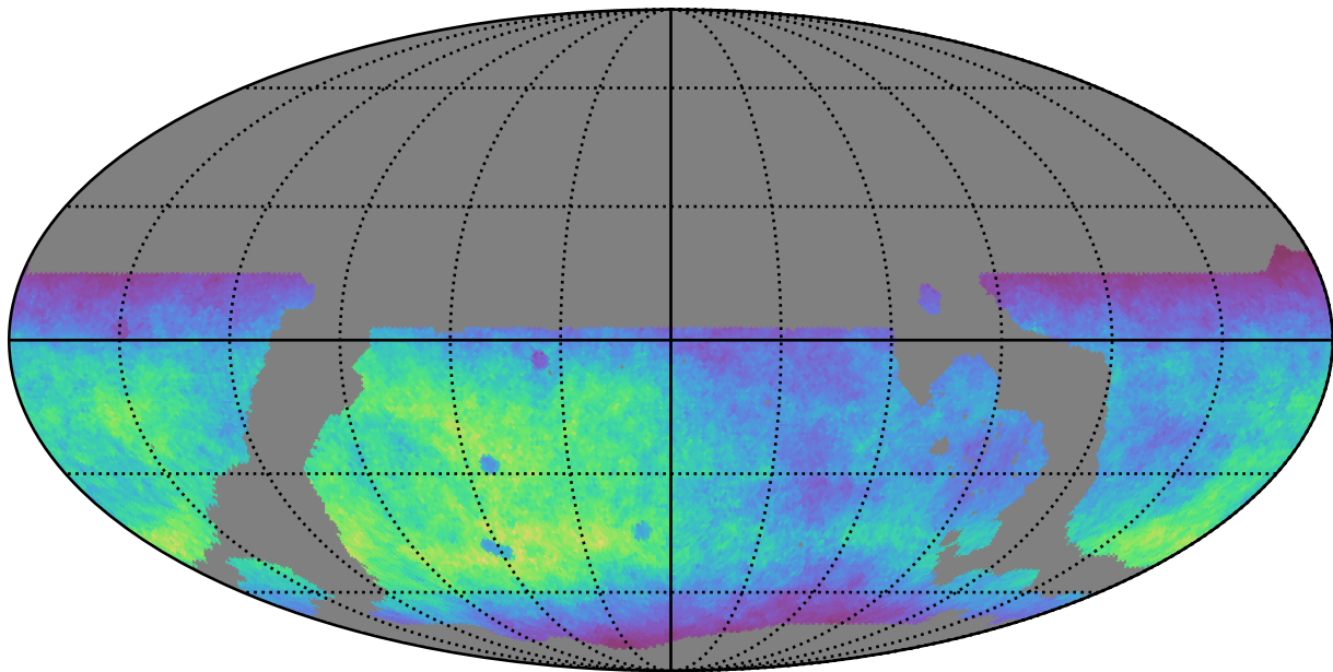
ddf_loaded_fl1_v3.4_10yrs WFD g band: Normalized Teff
