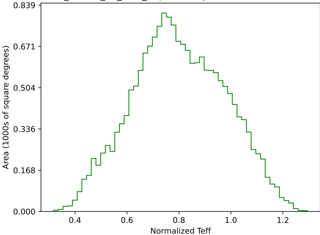
ddf_loaded_fl1_v3.4_10yrs WFD g band: Normalized Teff
