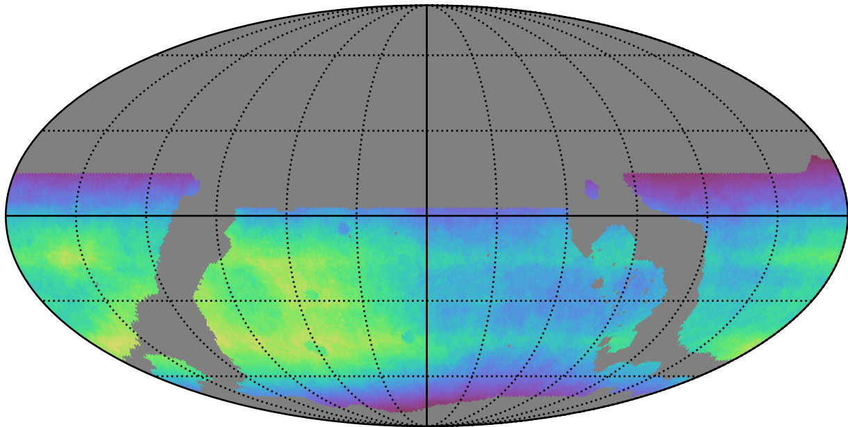
ddf_loaded_fl1_v3.4_10yrs WFD all bands: Normalized Teff
