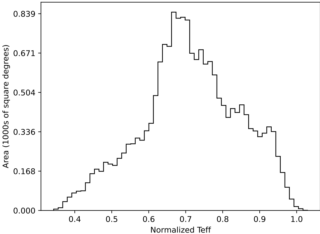
ddf_loaded_fl1_v3.4_10yrs WFD all bands: Normalized Teff
