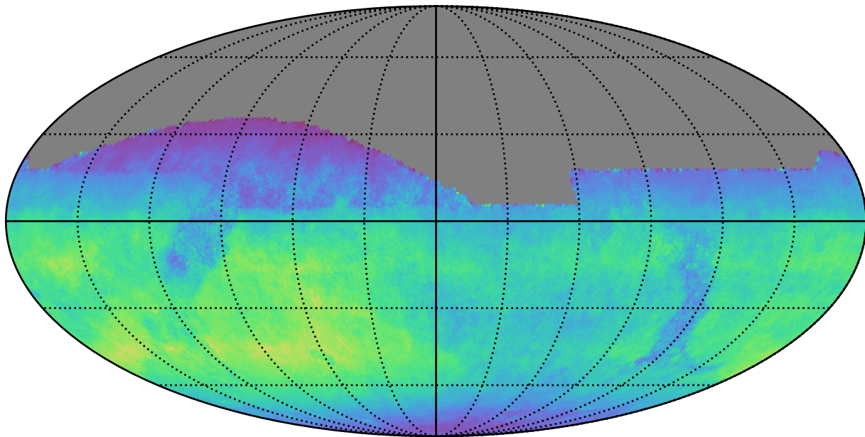
ddf_loaded_fl1_v3.4_10yrs All sky z band: Normalized Teff
