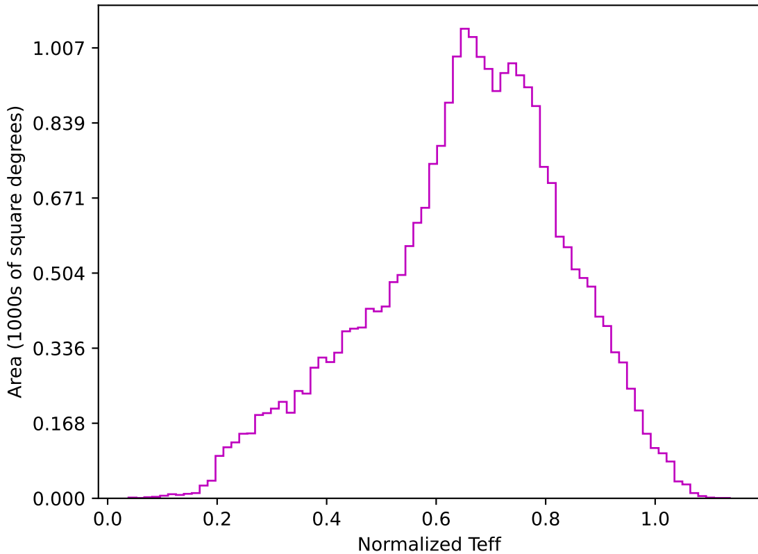
ddf_loaded_fl1_v3.4_10yrs All sky z band: Normalized Teff
