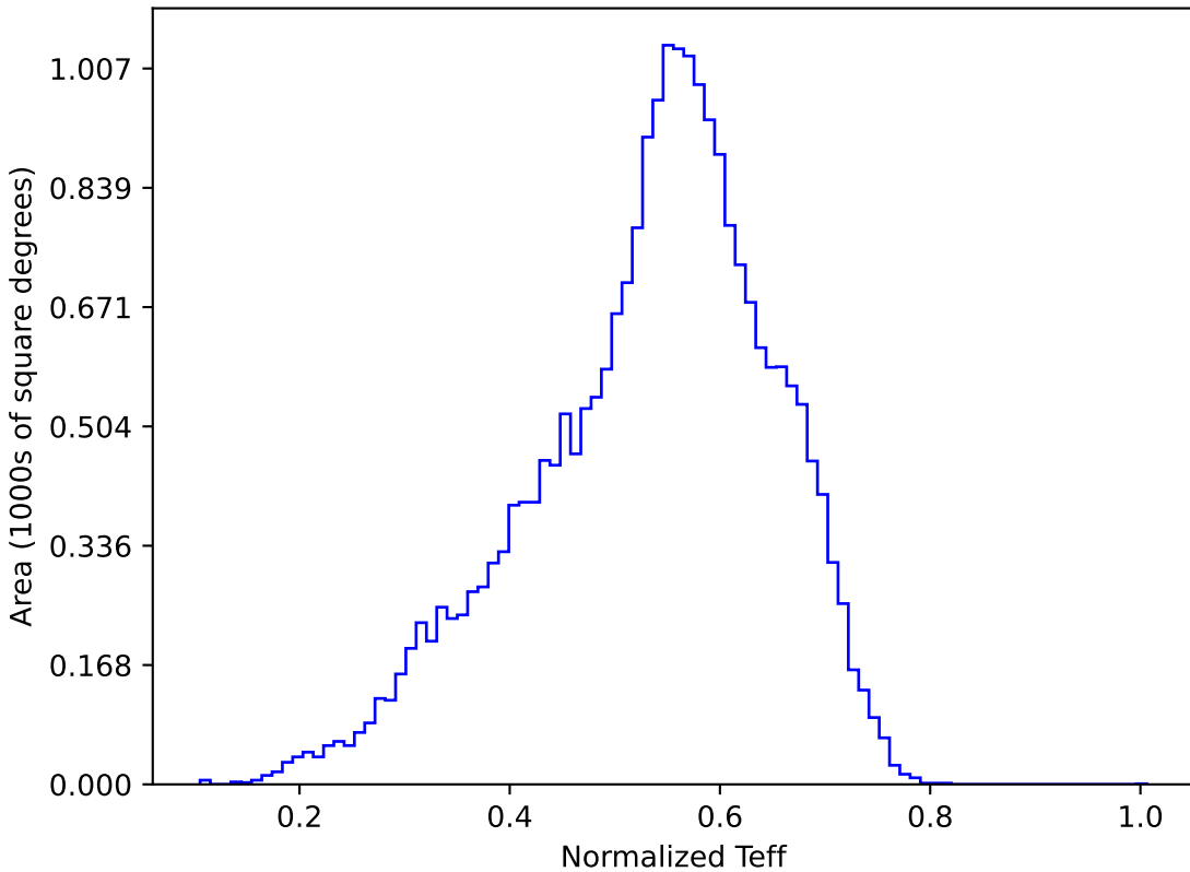
ddf_loaded_fl1_v3.4_10yrs All sky y band: Normalized Teff
