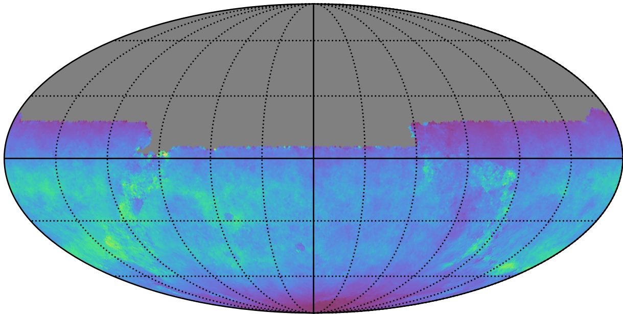
ddf_loaded_fl1_v3.4_10yrs All sky u band: Normalized Teff
