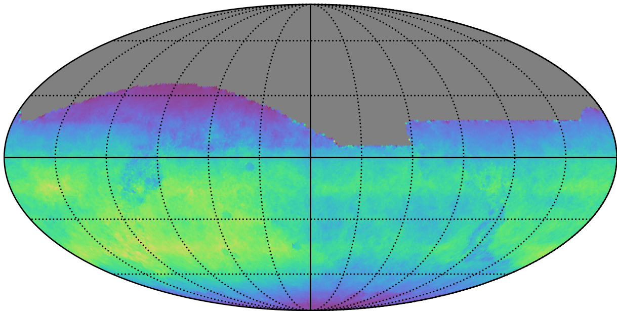
ddf_loaded_fl1_v3.4_10yrs All sky i band: Normalized Teff
