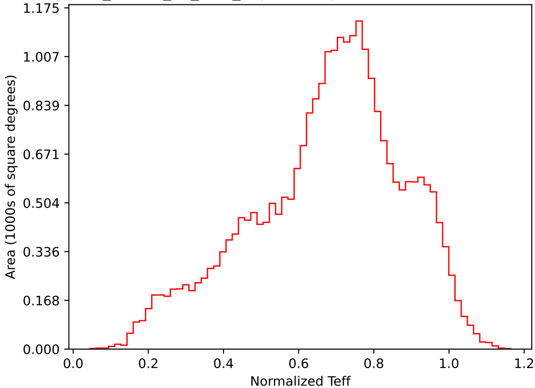
ddf_loaded_fl1_v3.4_10yrs All sky i band: Normalized Teff
