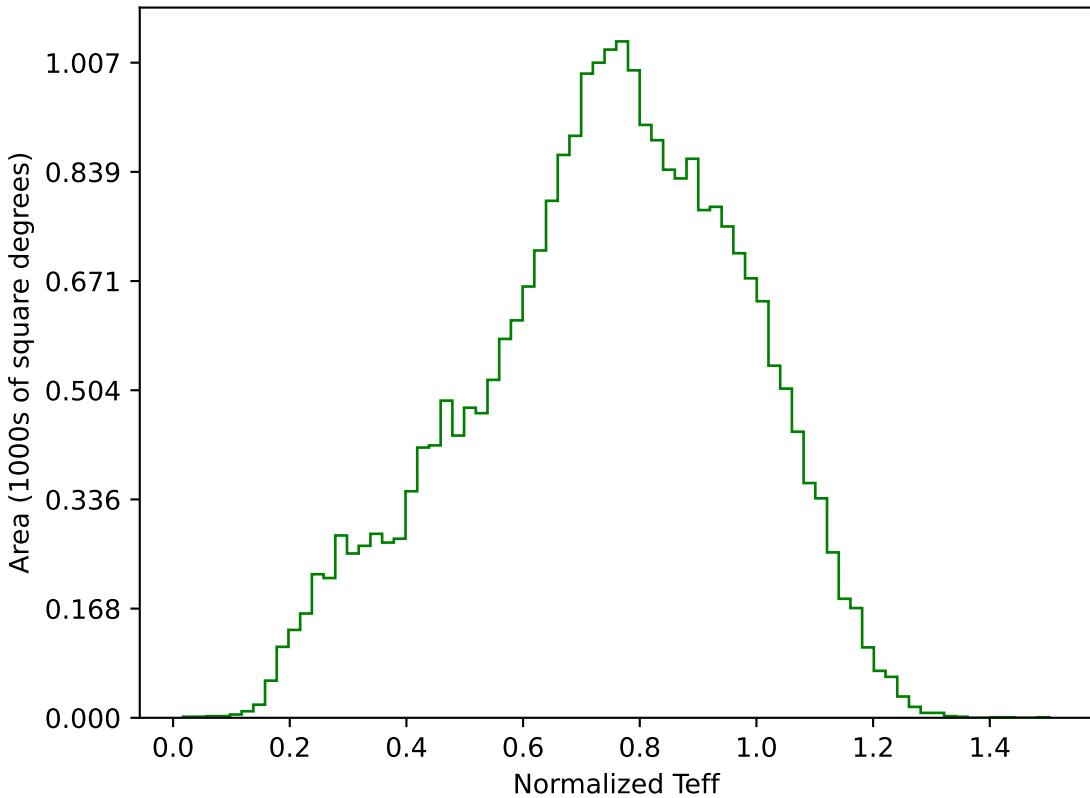
ddf_loaded_fl1_v3.4_10yrs All sky g band: Normalized Teff
