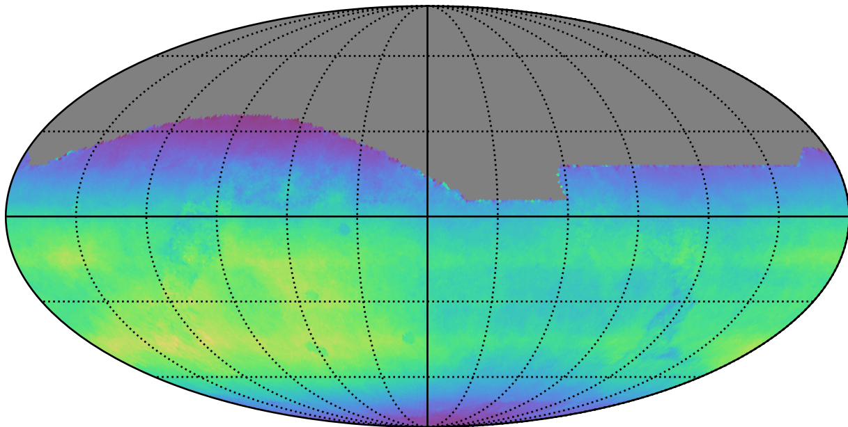
ddf_loaded_fl1_v3.4_10yrs All sky all bands: Normalized Teff
