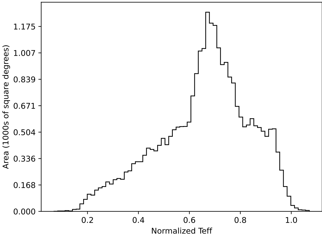
ddf_loaded_fl1_v3.4_10yrs All sky all bands: Normalized Teff
